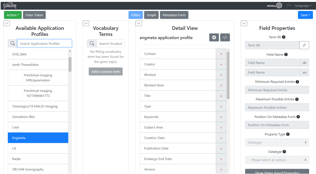
Figure 4: Screenshot of the application profile generator developed within AIMS [14].
